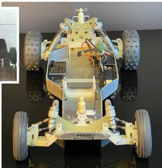
The prototype RC10 (right) and the full-size off-road buggy that inspired Roger Curtis for the design and box art.
